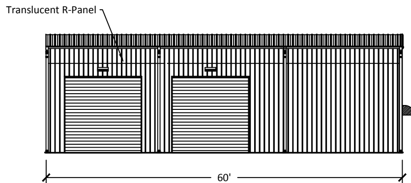
North Elevation
